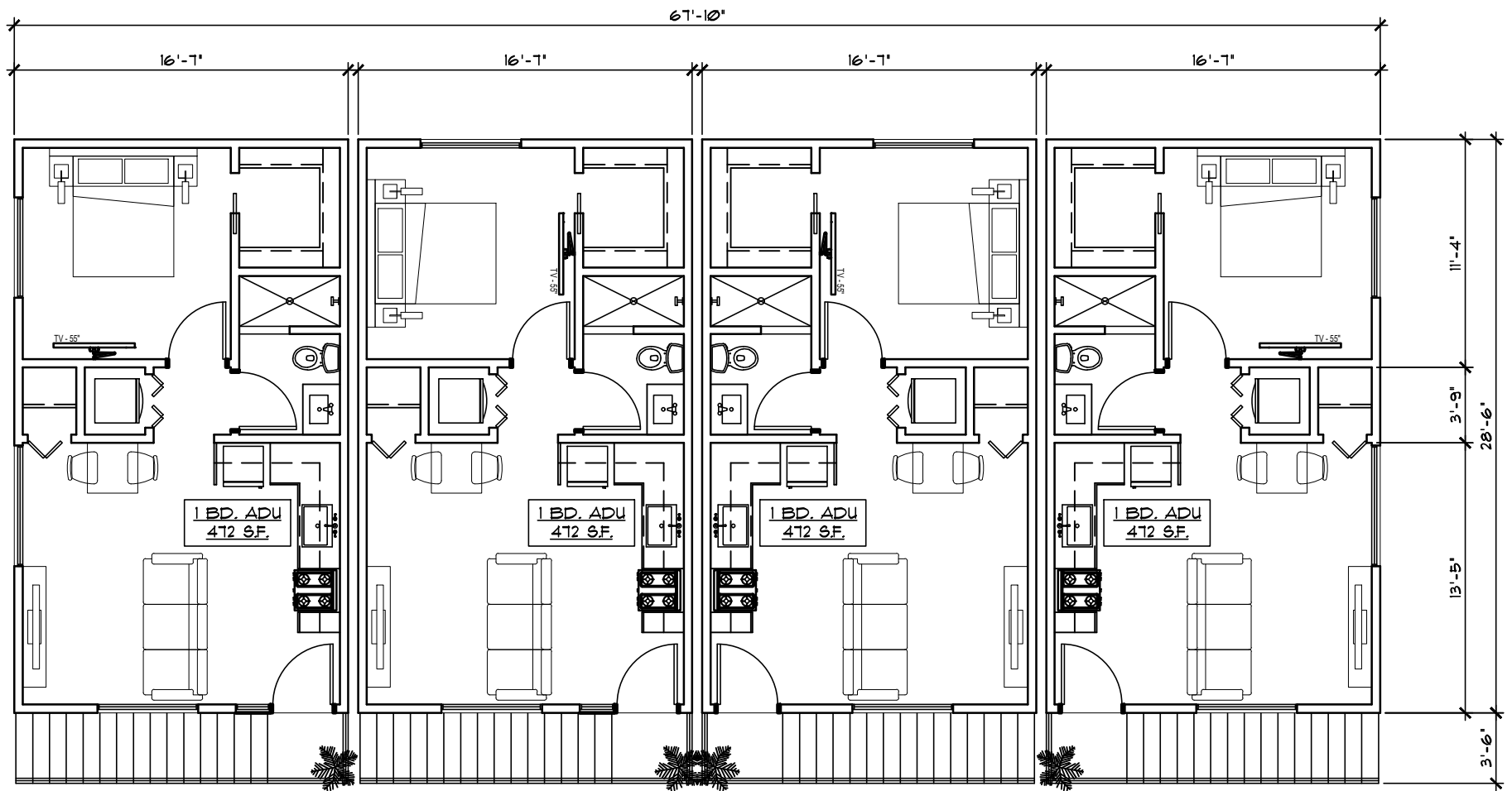
FLOOR PLAN 2ND FLOOR
